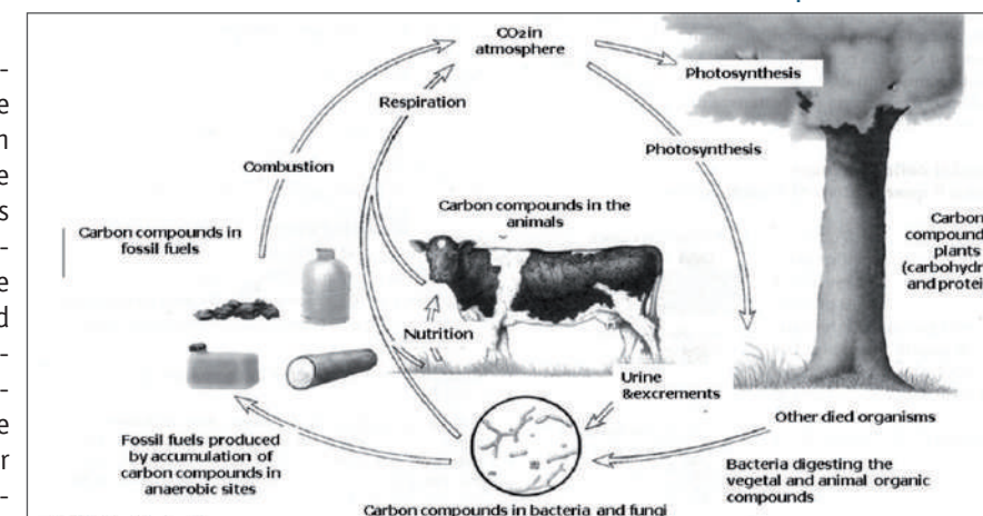
Figure 1 The carbon cycle ( http://web.ticino.com/gfwp/scuola/oss_2_co2.pdf )
