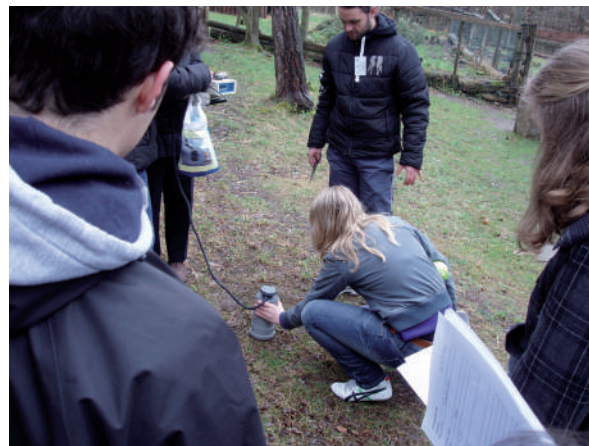
Measuring soil respiration
