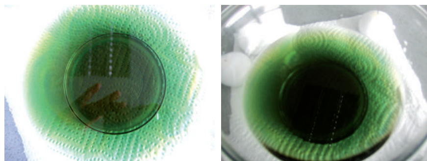
Colour of the water before and after the experiment with the lighted candles.
