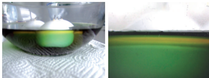
Some minutes after the candles are extinguished, a thin yellow layer of water forms at the surface. This indicates acidification of the surface layer because of dissolved carbon dioxide.
