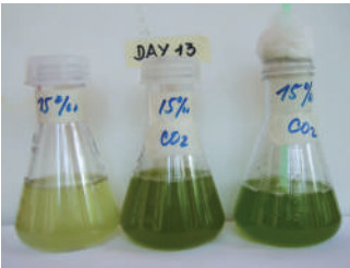
Carbon dioxide fertilization of marine microalgae ( Dunalliella sp.) cCultures
