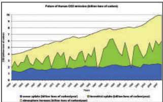
Global carbon budget between 1958 and 2008
