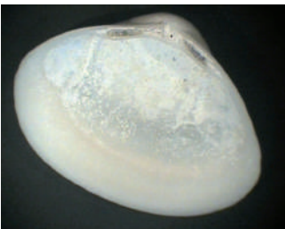
Atmospheric CO 2 can produce ocean acidification
